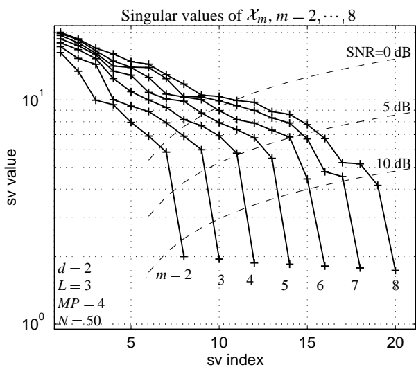
Fig. 3. Singular values of \mathcal{X}_m (noise-free), for a range of m . The dashed lines indicate which singular values will be masked by the noise.
