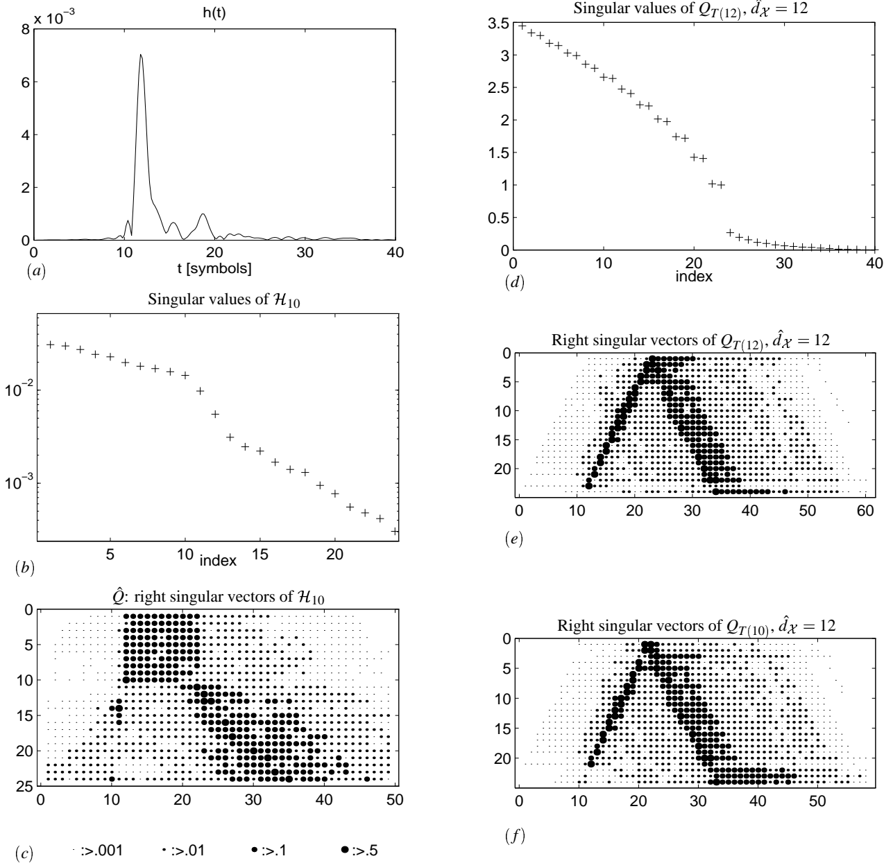
Fig. 6. (a) Channel impulse response h(t) , (b) singular values of \mathcal{H}_{10} : the numerical rank of \mathcal{H}_{10} is about 12, (c) \hat{Q} , i.e., right singular vectors of \mathcal{H}_{10} (magnitude of entries), (d) singular values of Q_{T(12)} , with \hat{d}_X = 12 , (e) right singular vectors of Q_{T(12)} , and (f) of Q_{T(10)}
