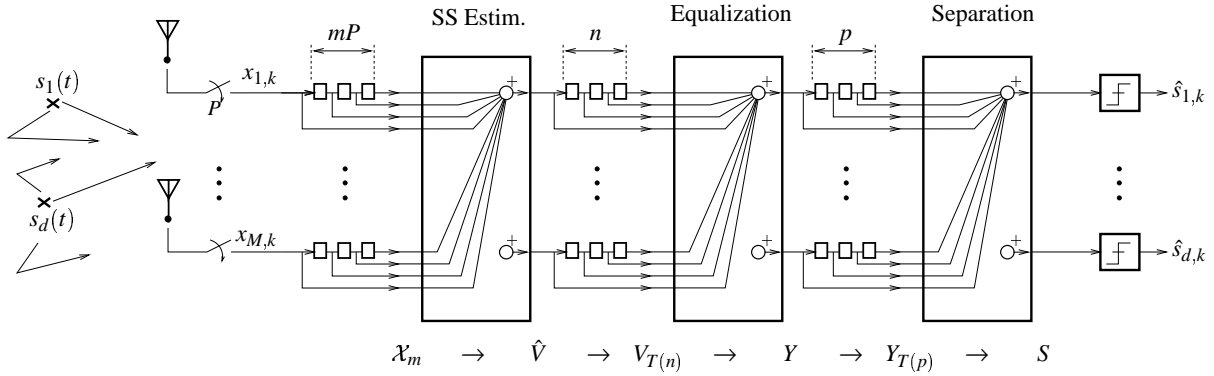
Fig. 2. Multistage equalization/separation filter
