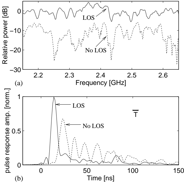
Fig. 7. (a) Relative power, and (b) response to a raised-cosine pulse ( T = 6 ns, \beta = 0.5 ) of two measured indoor channels
