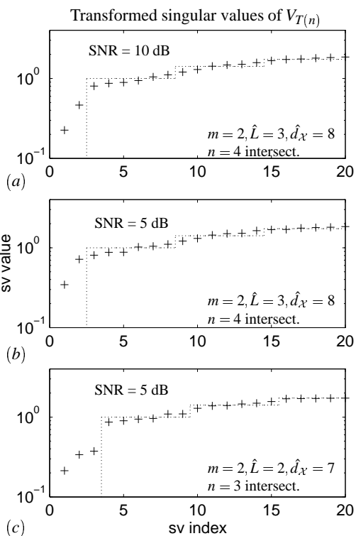
Fig. 4. Transformed singular values of V_{T(n)} , namely (n - \text{sv}(V_{T(n)})^2)^{1/2} . Small values indicate the number of remaining signals after intersections. (a) SNR = 10 dB, full intersections, (b) SNR = 5 dB, full intersections, (second source not resolved), (c) SNR = 5 dB, underestimating d_X and taking less intersections. After intersections, \hat{d}_S = 3 signals remain.
