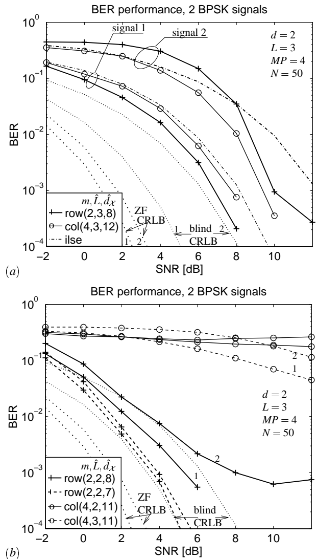
Fig. 5. BER performance for d = 2 BPSK signals, (a) using exact values \hat{L} = L , \hat{d}_X = d_X = d(L + m - 1) , (b) using approximate values. For comparison, indicated is the CRLB for a zero-forcing equalizer ( \mathcal{H}_N^* ), assuming perfect knowledge of H , the CRLB for the blind scenario (not using the FA property), and the performance of ILSE initialized with the exact H .
