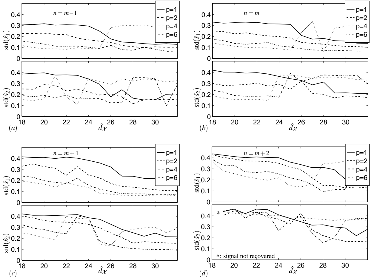
Fig. 9. Standard deviations of signal estimates, for m = 7 and varying settings of \hat{d}_x , n , p .
