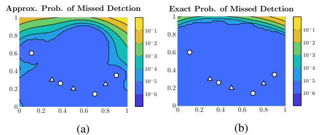
Fig. 2: Comparison of (a) approximate and (b) the exact probability of missed detection. The transmitters are denoted by circles and the receivers by triangles. The approximation produces slightly larger probability of missed detection.
