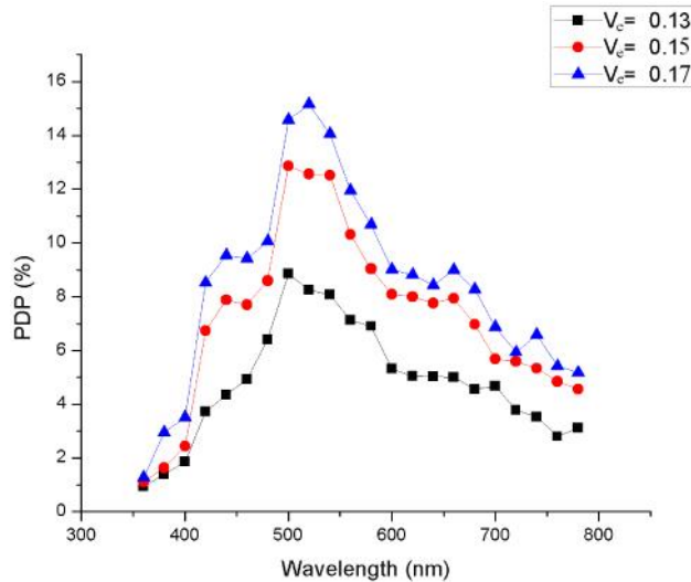
Fig. 7. Photon Detection Probability (PDP) at room temperature.
