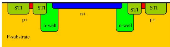
Fig. 1. Cross-section of one of the structures implemented for this family of SPADs.
